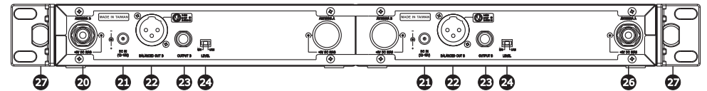
ACT-311BT/ACT-311T Dual Channel (Detachable 1/2 Wave Antenna ×2)
